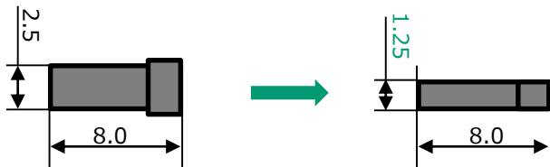
Half Thickness MT Ferrule
